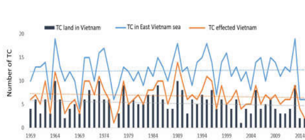
Figure 5. Evolution of typhoons and tropical depressions in the period 1959-2014
