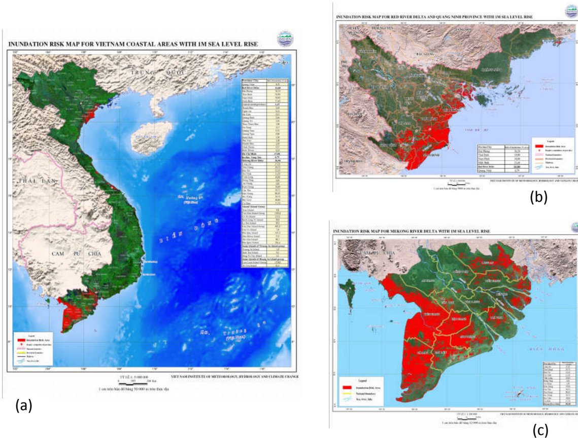
Figure 20. Inundation maps with a sea level rise of 100 cm
